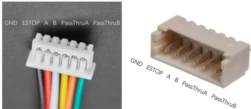
图 7: BEAR Signal Port Pinout
